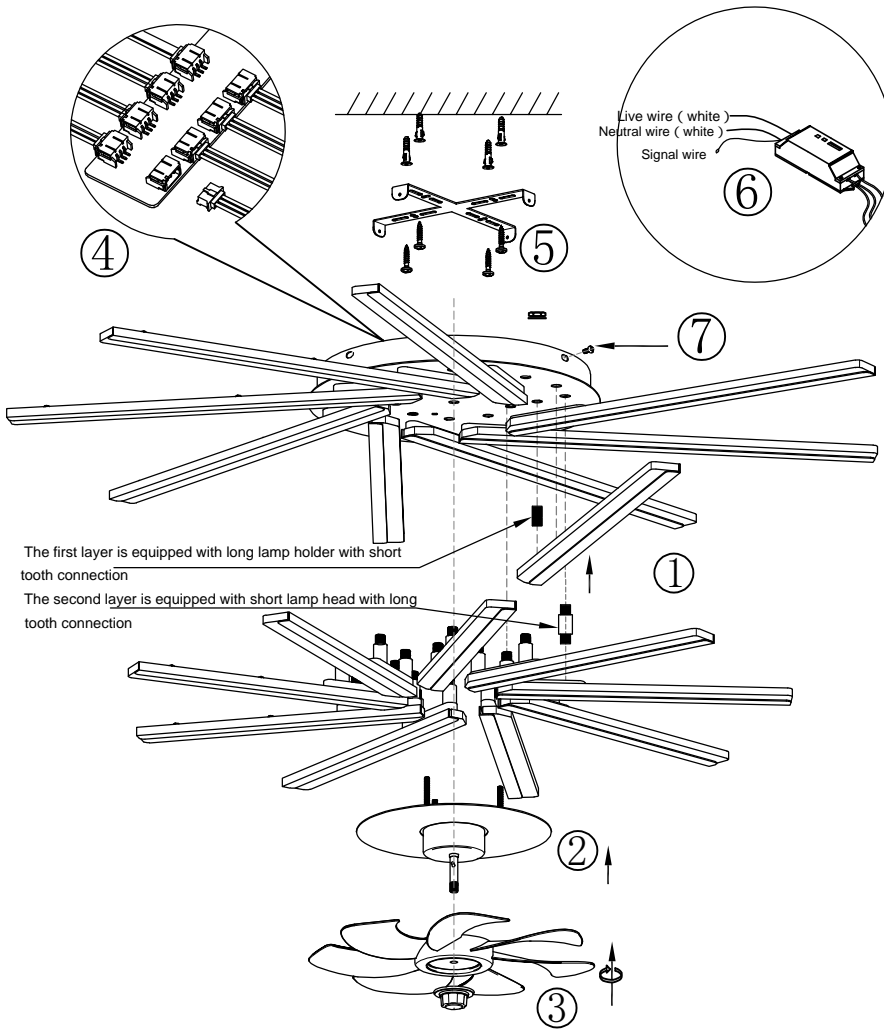
9+9 Display diagram
